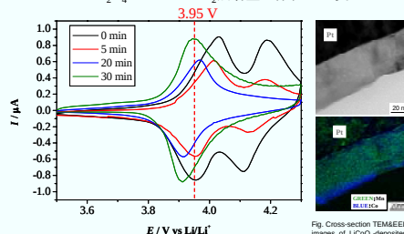
Fig. Potential sweep curves for the Li/LiPON/LiCoO 2 -deposited LiMn 2 O 4 batteries at R.T.
