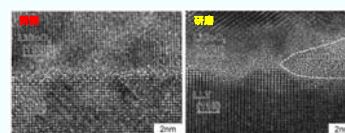
Fig. TEM image of Lanthanum titanium oxide/lithium cobalt oxide interface.
